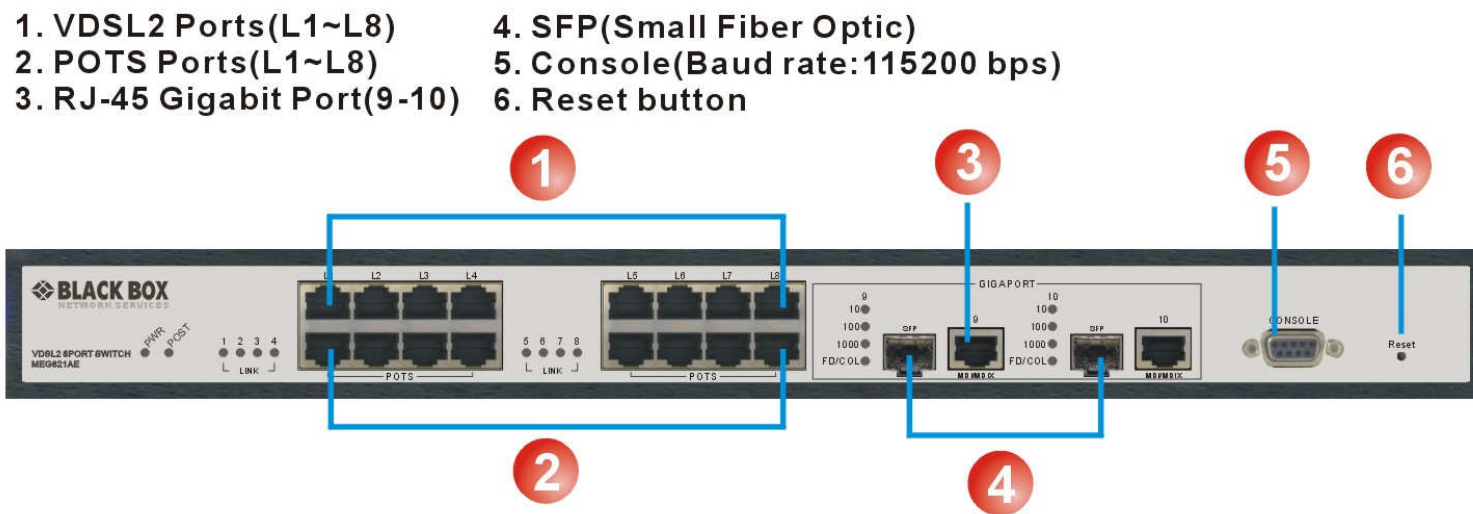
Figure 2-1 Front Panel description
